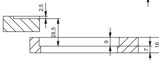
Material thickness 16mm Materialstärke 16mm
