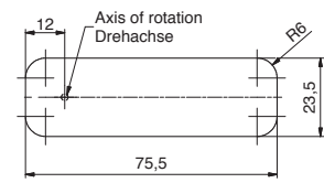
Stamping configuration, glass / steel Stanzbild, Glas / Stahl 0,8 – 3 mm
